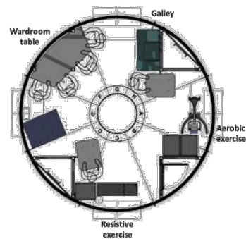
HDU-DSH Upper Level Plan
