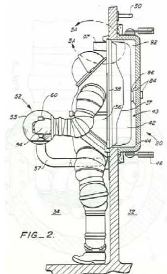
FIGURE 7a. Cross-Section through the Suitport. US Patent 4,842,224.
