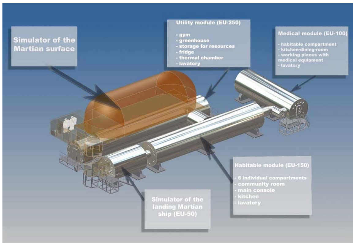
FIGURE 15. Isometric view of the EuroMars 500 Simulator configuration at the Institute for Biomedical Problems (IBMP), Moscow. Courtesy of ESA.
